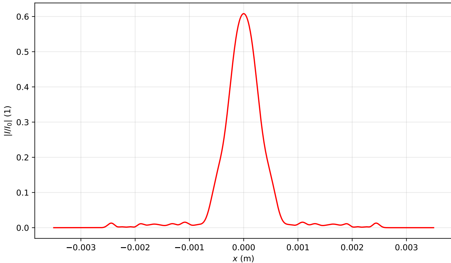
Intensity profile I(x, y = 0, z = 3.582)/I_0 , P_{in}=3.0P_{cr} , artificial time
